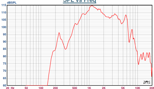
Sound pressure levels at 1W/1m TUNNEL500/DUP-40
